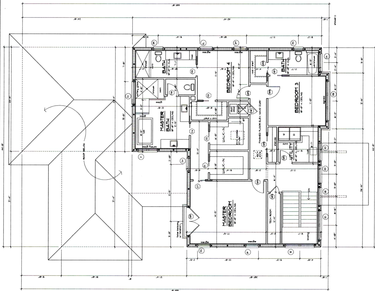
FLOOR PLAN-SECOND FLOOR 1638 S.F.
